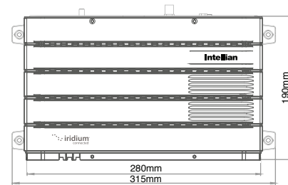
Stand-Alone Type BDU
